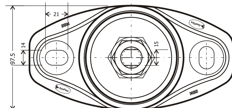
M85-20S General Arrangement
