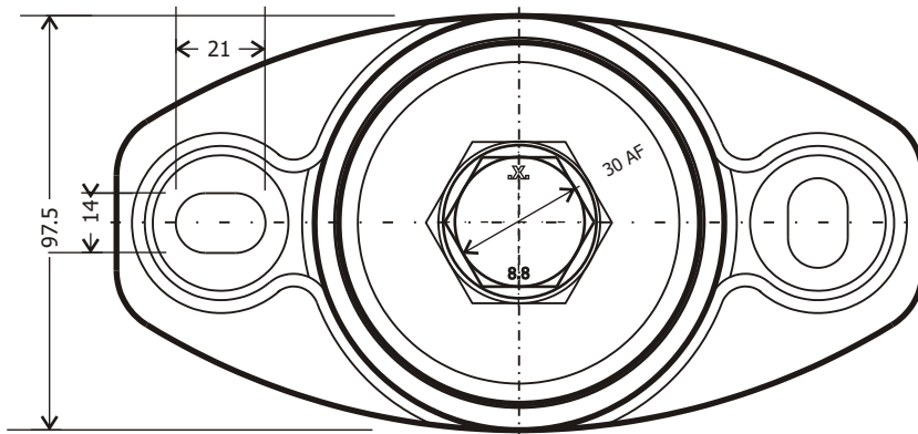
M80-20B-General Arrangement
