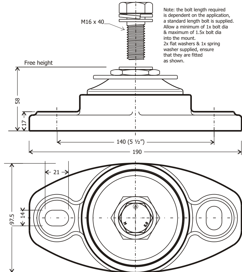
M80-16B-General Arrangement
