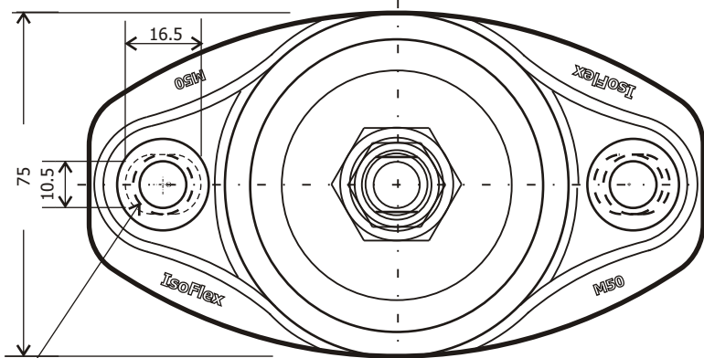
M50-12 General Arrangement
