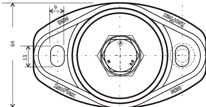
IsoFlex Mount Model Number: M30-12B
