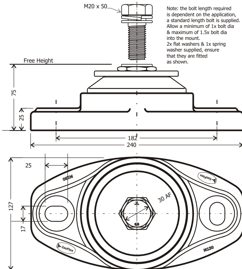
M130HD-20B General Arrangement
