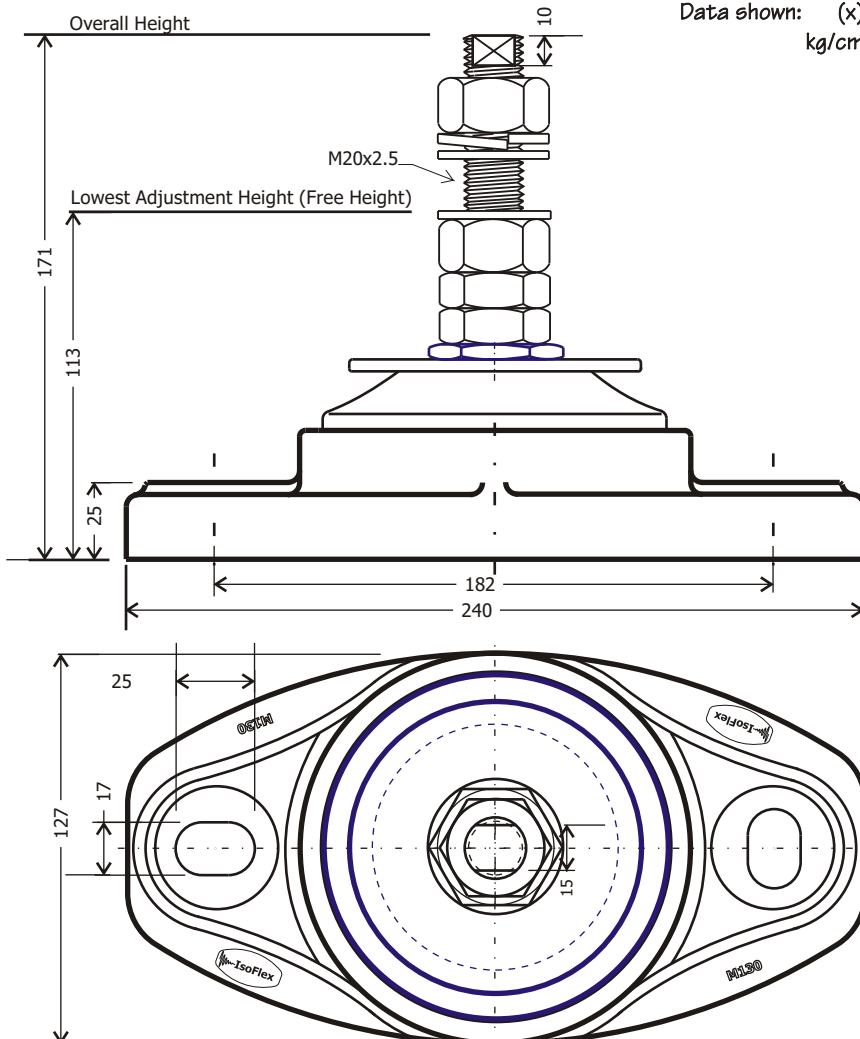
M130-20S General Arrangement
