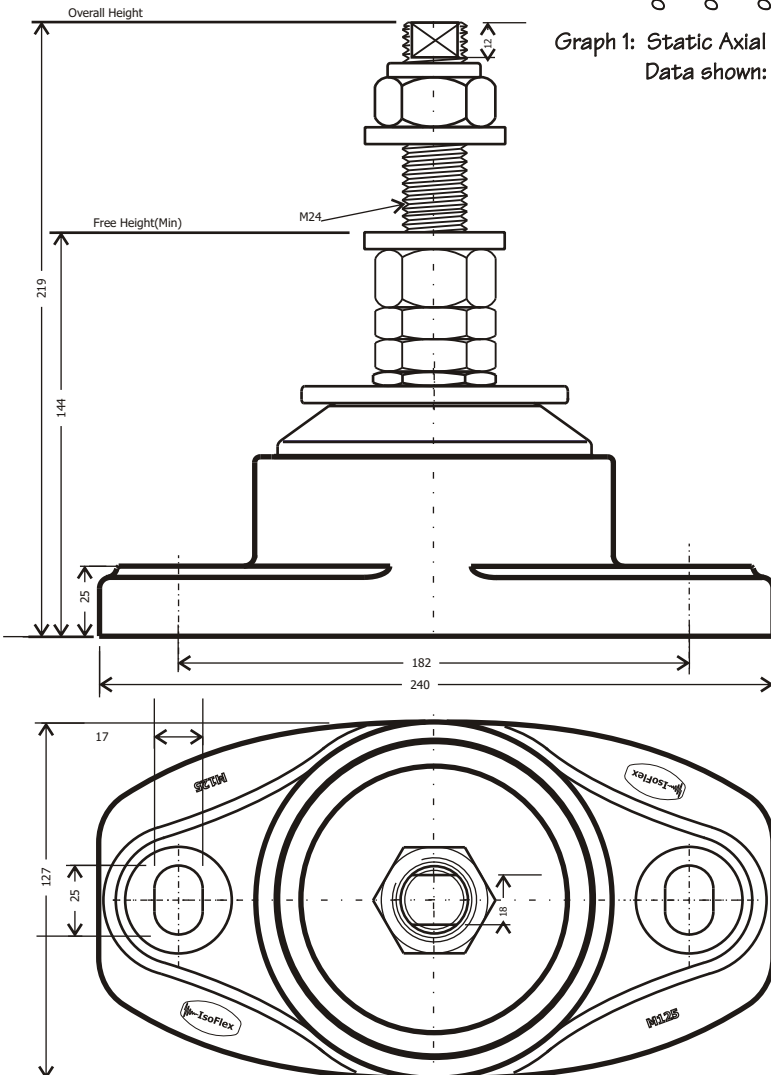
M127HD-24S General Arrangement
