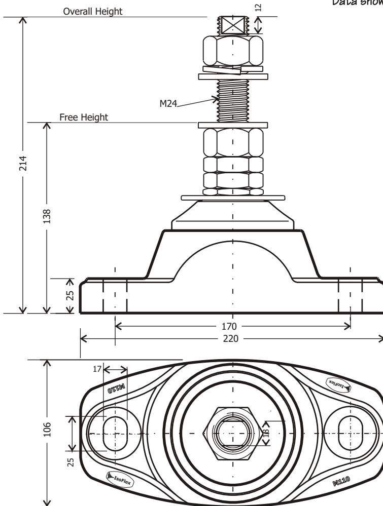
M110-24S General Arrangement
