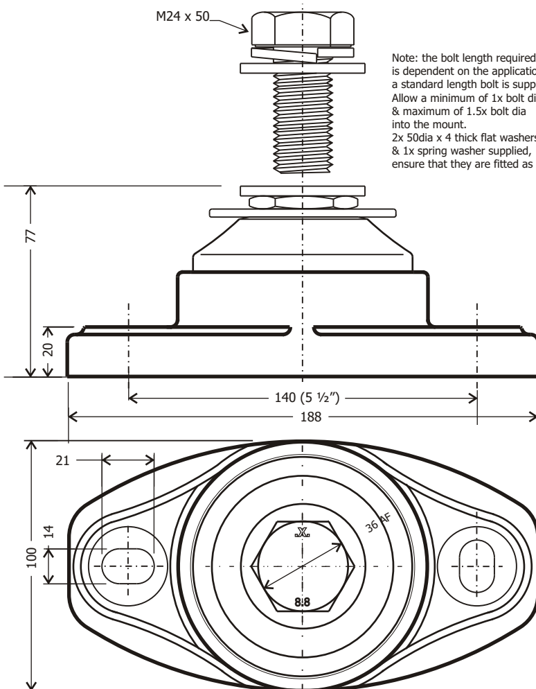
M100-24B General Arrangement
